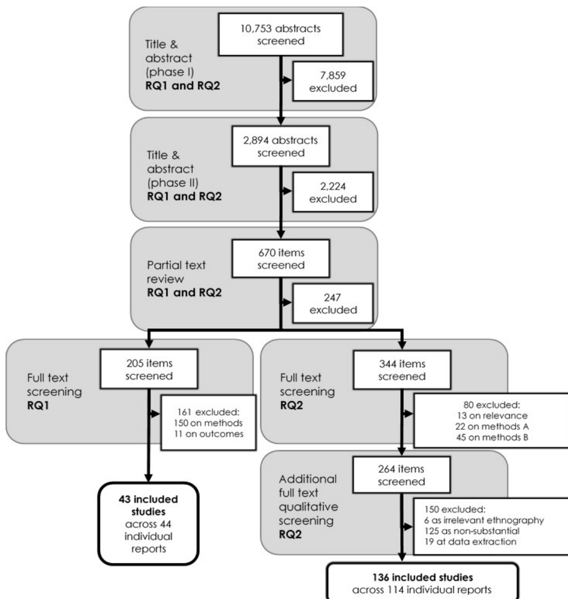
Figure 6: PRISMA diagram
